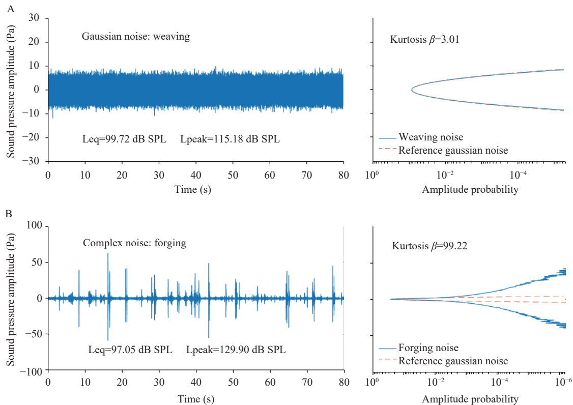
FIGURE 1. Waveforms (left) and amplitude probabilities (right) from two industrial noises: (A) steady-state noise; (B) non-steady (complex) noise. Red lines, background Gaussian noise probabilities.
