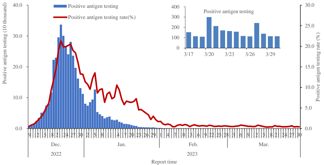
Figure 1-2 COVID-19 antigen test and positive rate (Data reported by PLADs in Chinese mainland)
