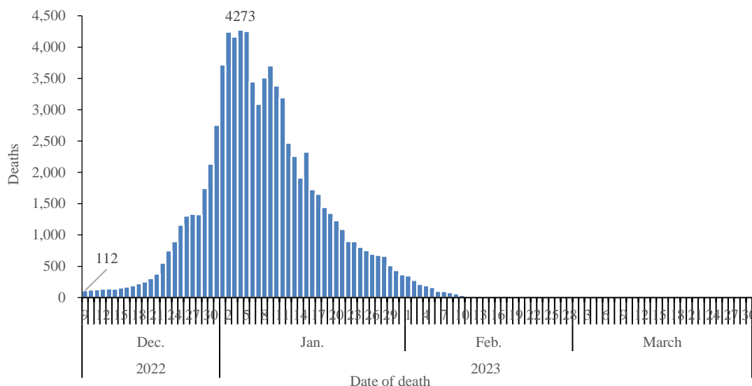
Figure 3-3 No. of deaths with SARS-CoV-2 in hospitals (Data reported by PLADs in Chinese mainland)
