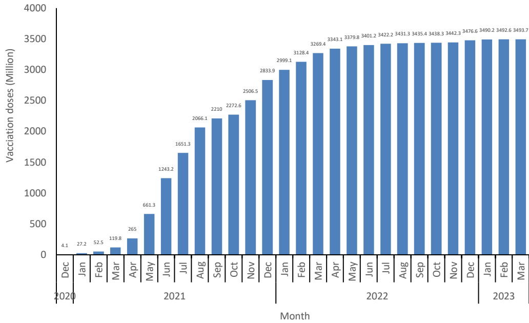
Figure 5-1 Cumulative COVID-19 Vaccine Doses Administered in China by Month. (Data reported by PLADs in Chinese mainland)
