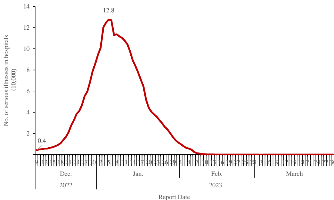
Figure 3-2 No. of severe cases in hospitals (Data reported by PLADs in Chinese mainland)
