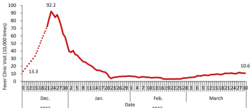
Figure 2-2 Trends of rural fever clinic visit data
