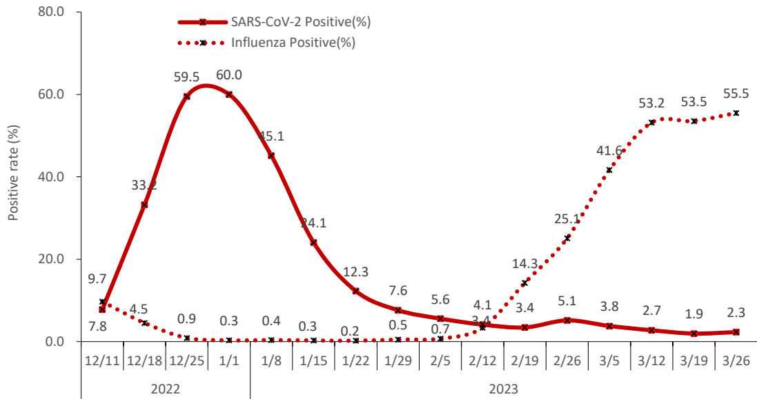
Figure 2-5 The positive rate of SARS-CoV-2 and influenza virus in ILI samples from sentinel hospitals in Chinese mainland (Reported data were from 402 laboratories)
