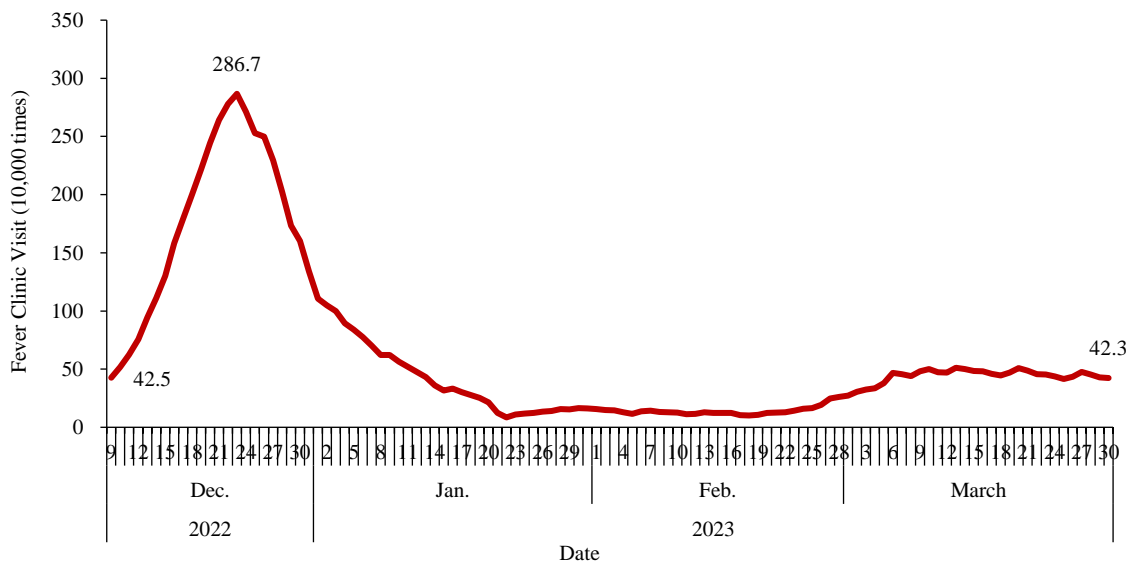
Figure 2-1 Trends of fever clinic visit data (Data reported by PLADs in Chinese mainland)
