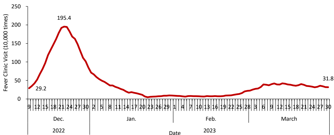
Figure 2-3 Trends of urban fever clinic visit data
